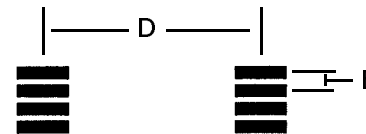
8 LEAD DEVICE FOOTPRINT
